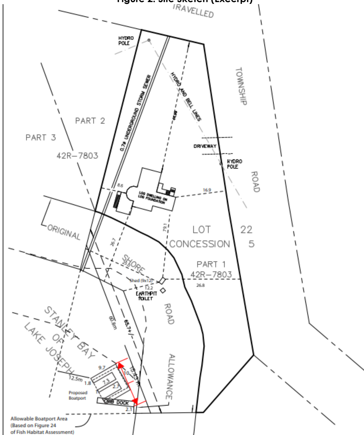
Figure 2: Site Sketch (Excerpt)
